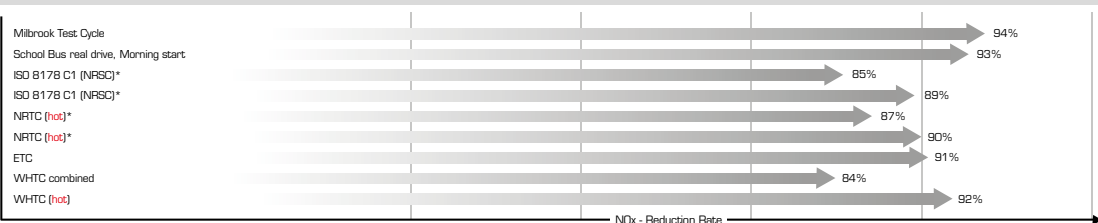
NO x reduction rate performed on test cycles with TDI-engines from 6L to 11L
